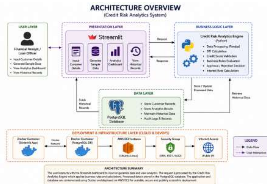
Figure (1): Smart Loan Approval System Architecture
